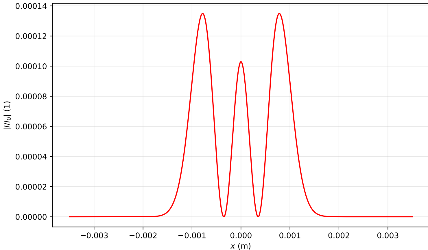
Intensity profile I(x, y = 0, z = 0.080)/I_0 , P_{in}=0.5P_{cr} , artificial time
